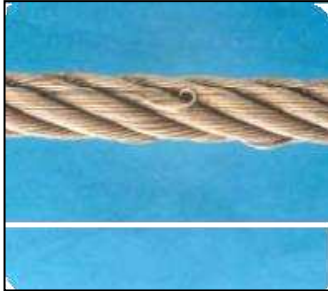
Damaged steel wire rope
